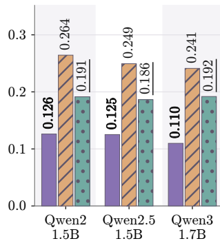
(c) DTW ↓
