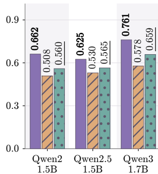
(e) Micro-F1 ↑
